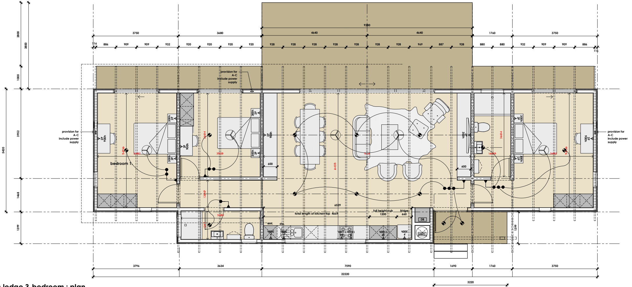
zim lodge 3-bedroom : plan
